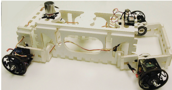
Fig. 6. SEAL Pack in Car State with Payload.
